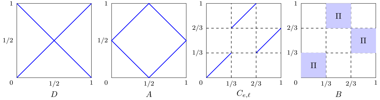
Figure 1: Supports of copulas D , A , C_{e,\ell} and B
